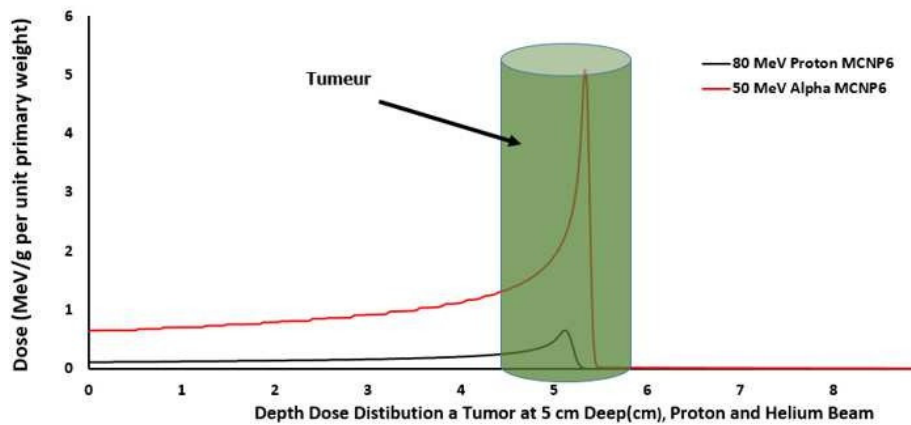
Figure 6: Depth-dose distribution of 80 MeV proton beam and 50 MeV helium beam in water calculated using MCNP6
