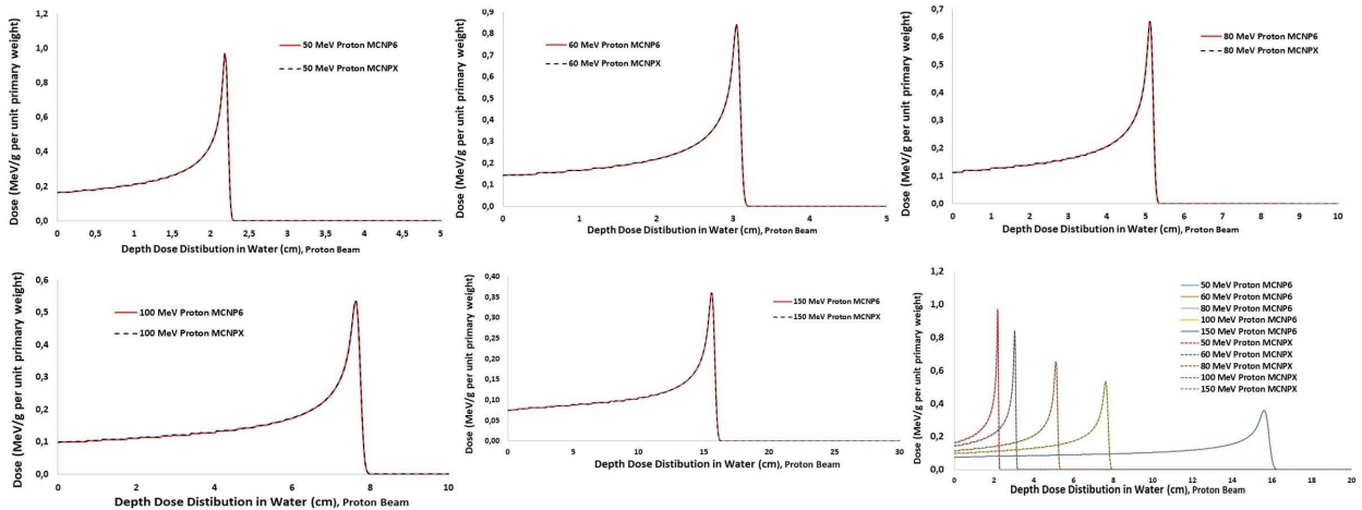
Figure 4: Depth-dose distribution of different proton beam energy in water calculated using MCNP6 and MCNPX
