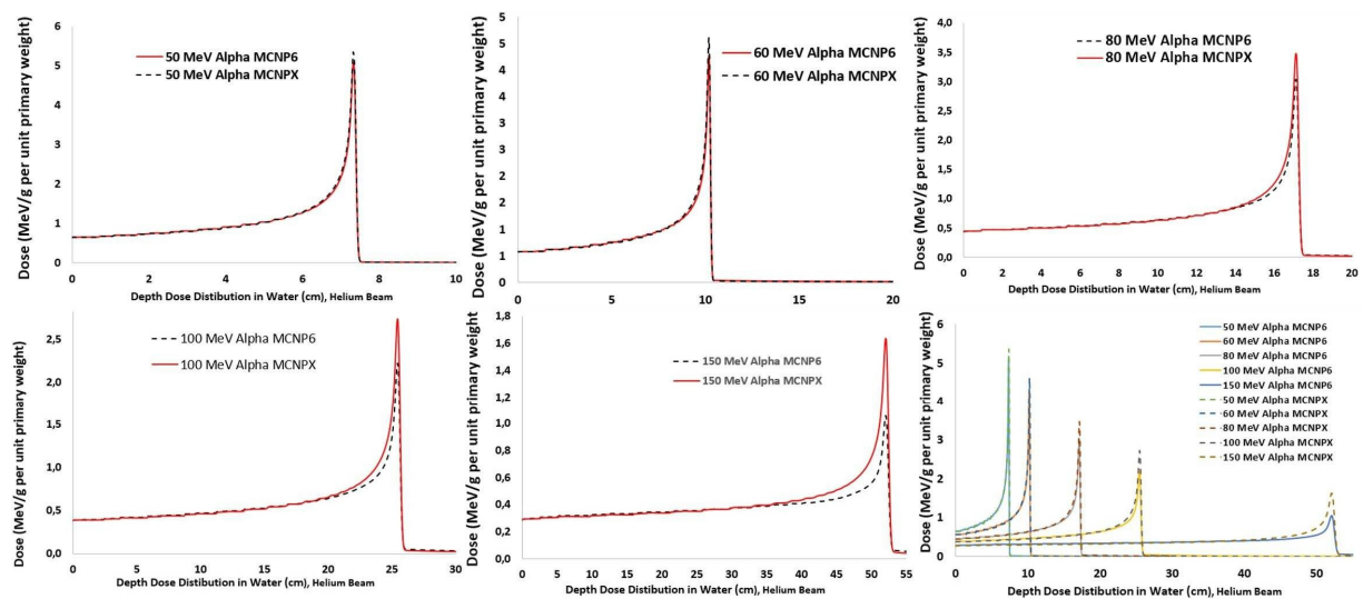
Figure 2: Depth-dose distribution of different helium Beam Energy in water calculated using MCNP6 and MCNPX
