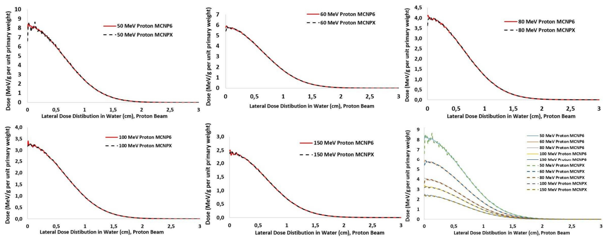
Figure 5: Lateral dose distribution of different proton beam energy in water calculated using MCNP6 and MCNPX
