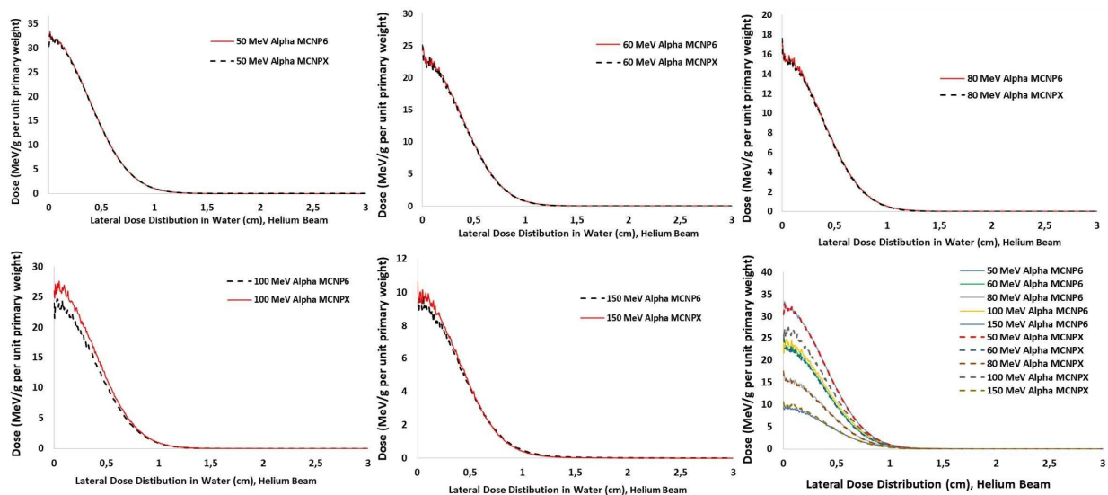
Figure 3: Lateral dose distribution of different helium beam energy in water calculated using MCNP6 and MCNPX
