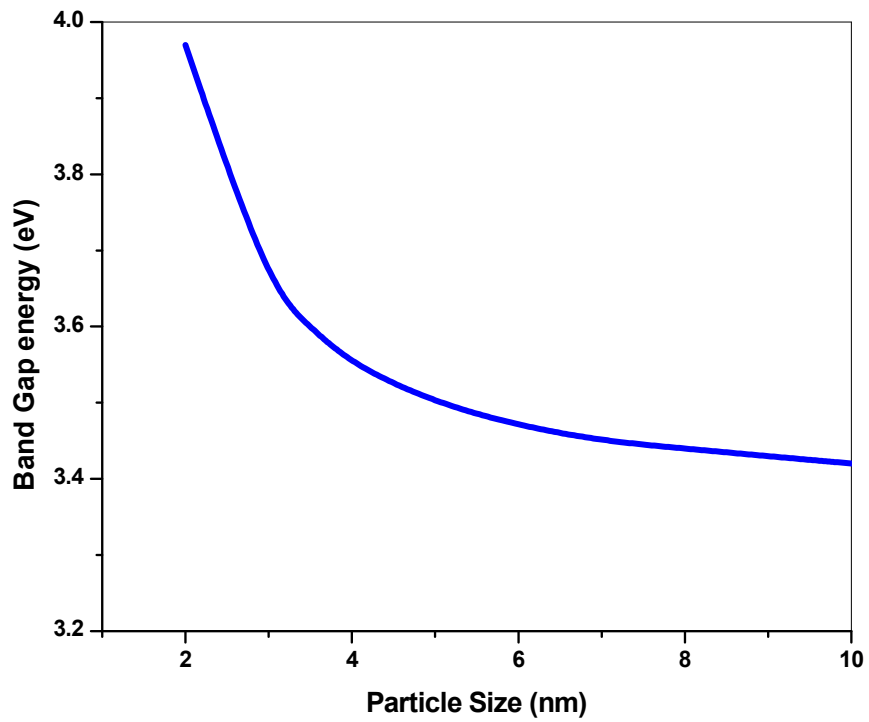
Figure-4: Variation of band gap energy with size of ZnO nanoparticles theoretically generated from effective mass model.
