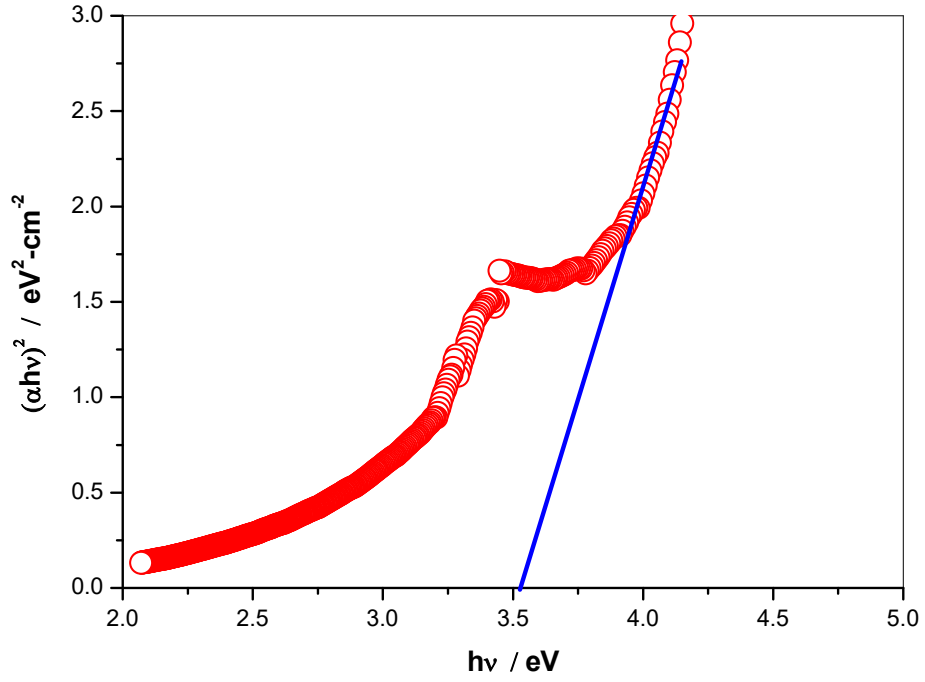
Figure-3: Tauc plot from UV-visible absorption spectrum to calculate band gap of synthesized ZnO nanoparticles.
