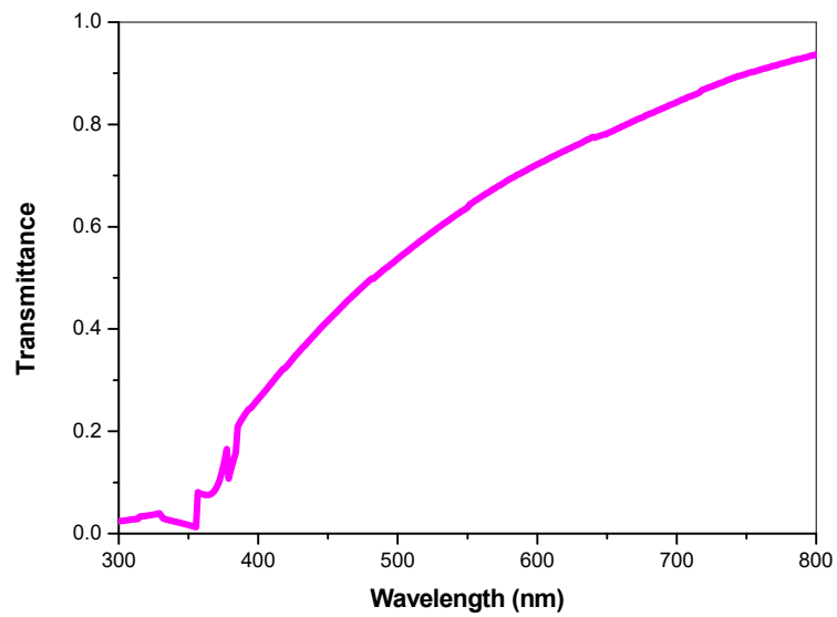
Figure-2: UV-visible transmission spectrum of synthesized ZnO nanoparticles.
